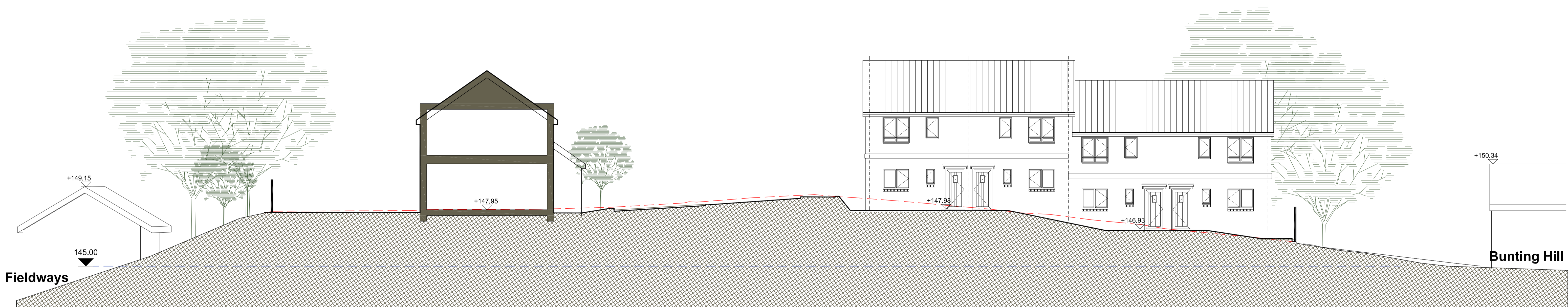
Block Section / Elevation B-B
