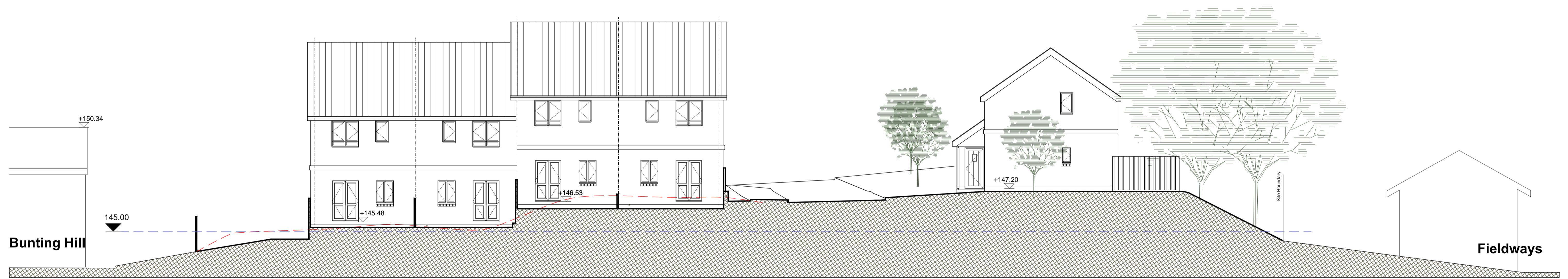
Block Section / Elevation D-D
